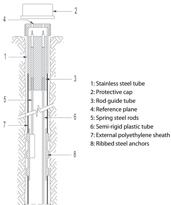
WR-FLEX Schematic
