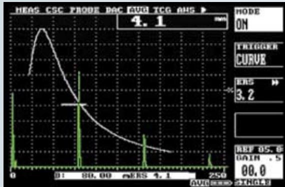
Curva AVG AVG curve
