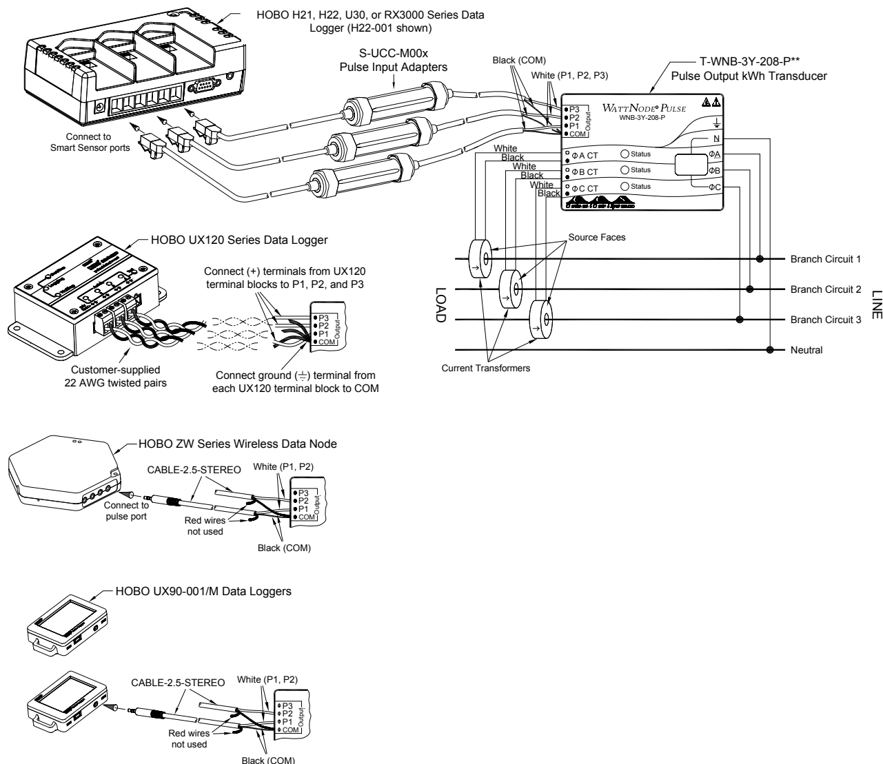
Figure 7: Separate Branch Circuits Connection
