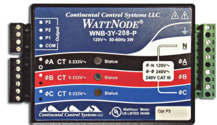
WattNode Pulse Output kWh Transducer (Onset Part No. T-WNB-3Y-208-P shown)
