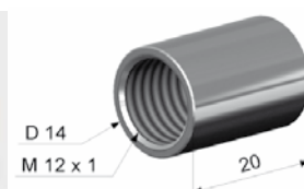
TM-PA-CT Pipe adapter for sighting tube
